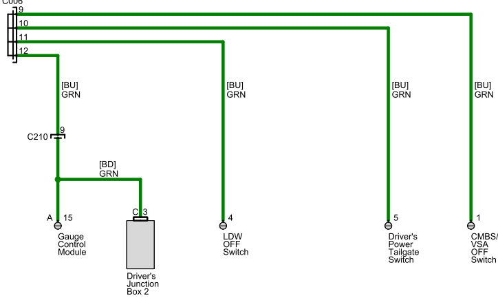
CR-V Junction Connectors 3 of 3
