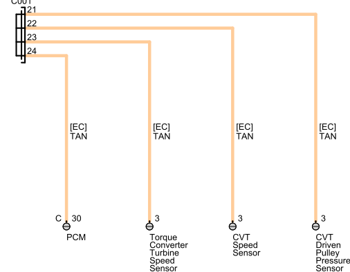
CR-V Junction Connectors 1 of 3
